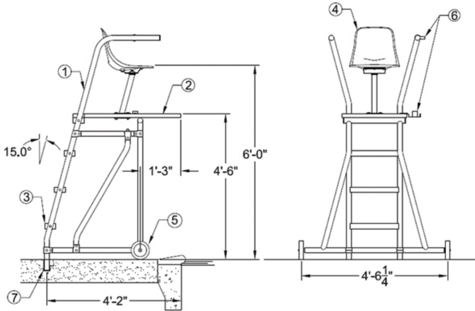
SIDE VIEW
